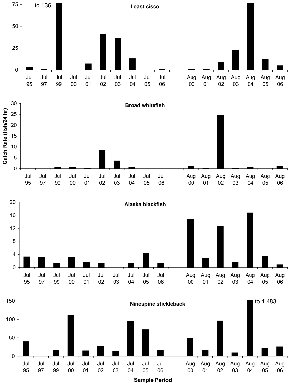
Figure 12. Mean catch rates of selected species in lake L9313, Alpine Development Area, 1995-2006 (* = nets fished in 1995 and 1997 were at different locations).
