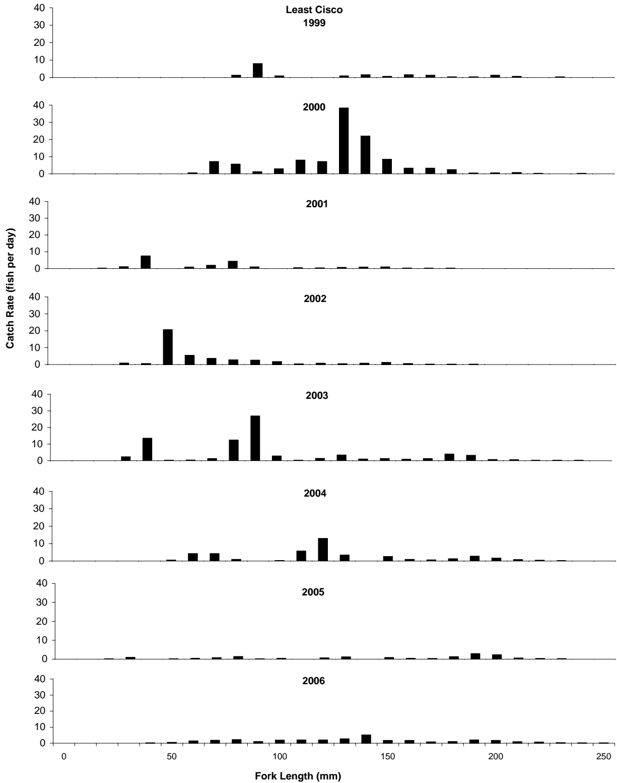
Figure 10. Length frequencies of least cisco in lake L9312 during 1999-2006 sampling with fyke nets.
